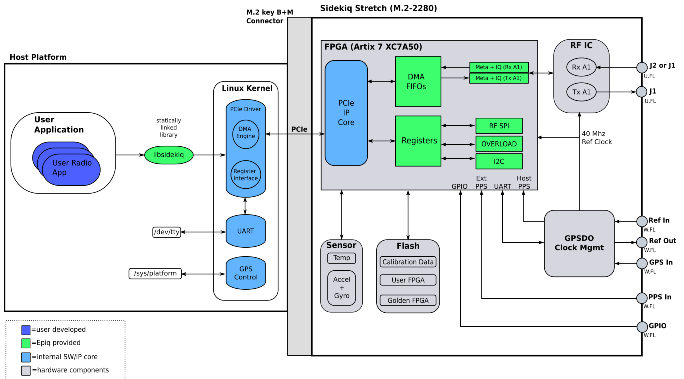
Fig. 4.3: Sidekiq Stretch block diagram showing how libsidekiq + user applications fit in the system
