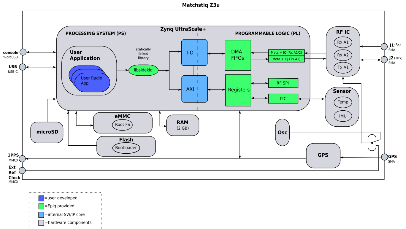
Fig. 4.9: Matchstiq Z3u block diagram showing how libsidekiq + user applications fit in the system
