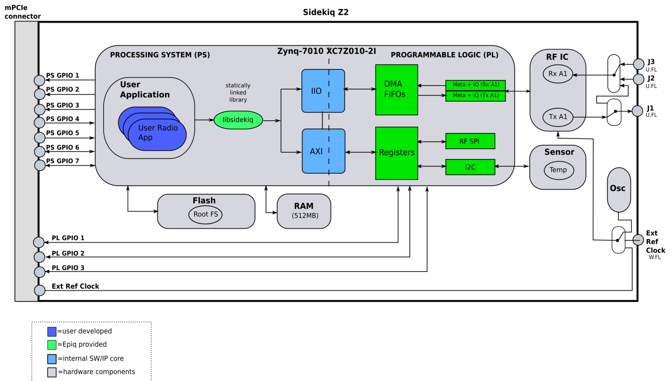
Fig. 4.8: Sidekiq Z2 block diagram showing how libsidekiq + user applications fit in the system
