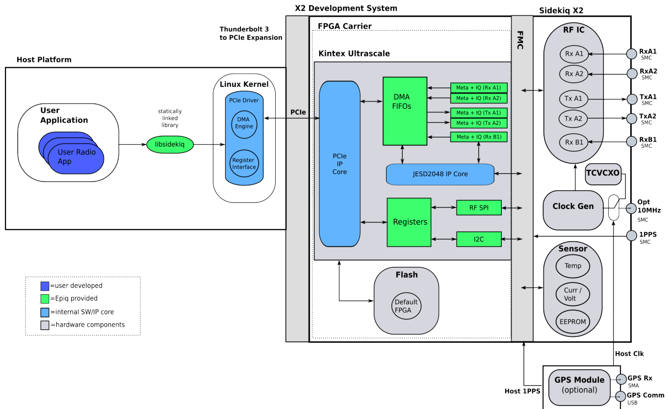
Fig. 4.6: Sidekiq X2 block diagram showing how libsidekiq + user applications fit in the system
