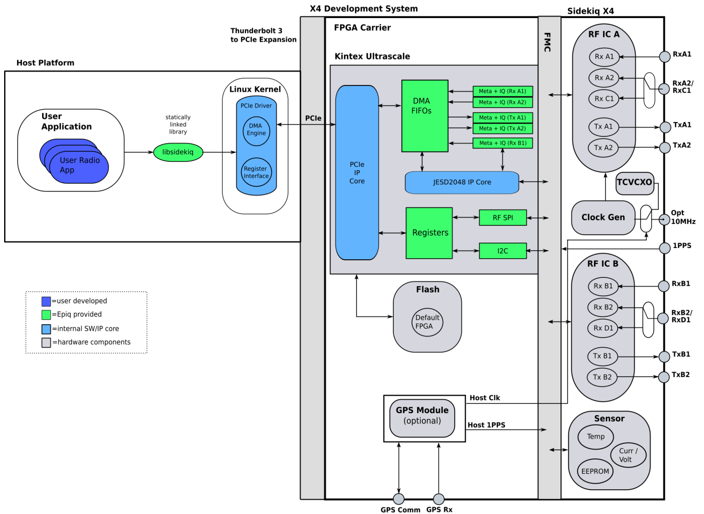
Fig. 4.7: Sidekiq X4 block diagram showing how libsidekiq + user applications fit in the system
