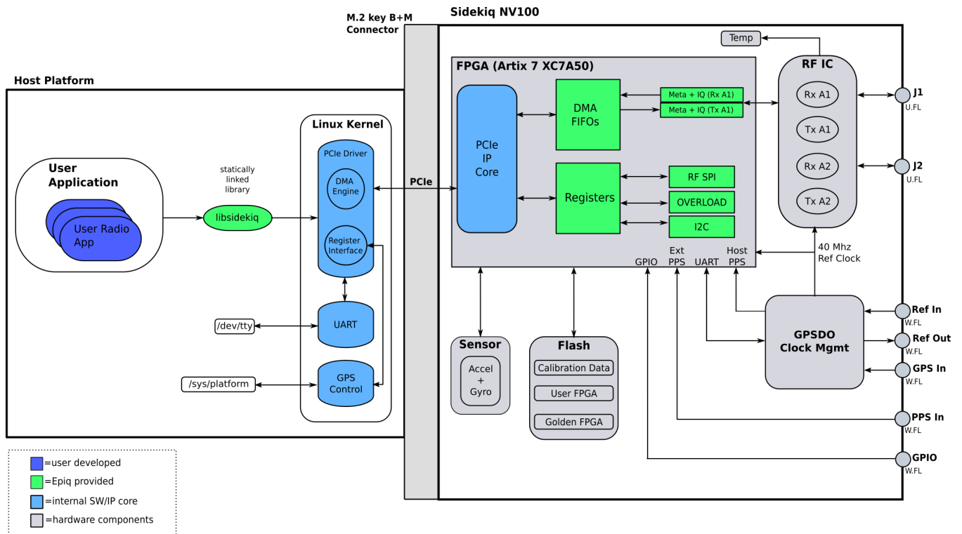
Fig. 4.4: Sidekiq NV100 block diagram showing how libsidekiq + user applications fit in the system
