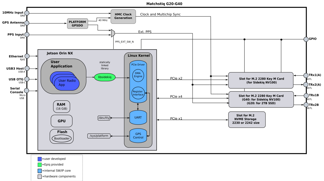
Fig. 4.10: Matchstiq G20-G40 block diagram showing how libsidekiq + user applications fit in the system
