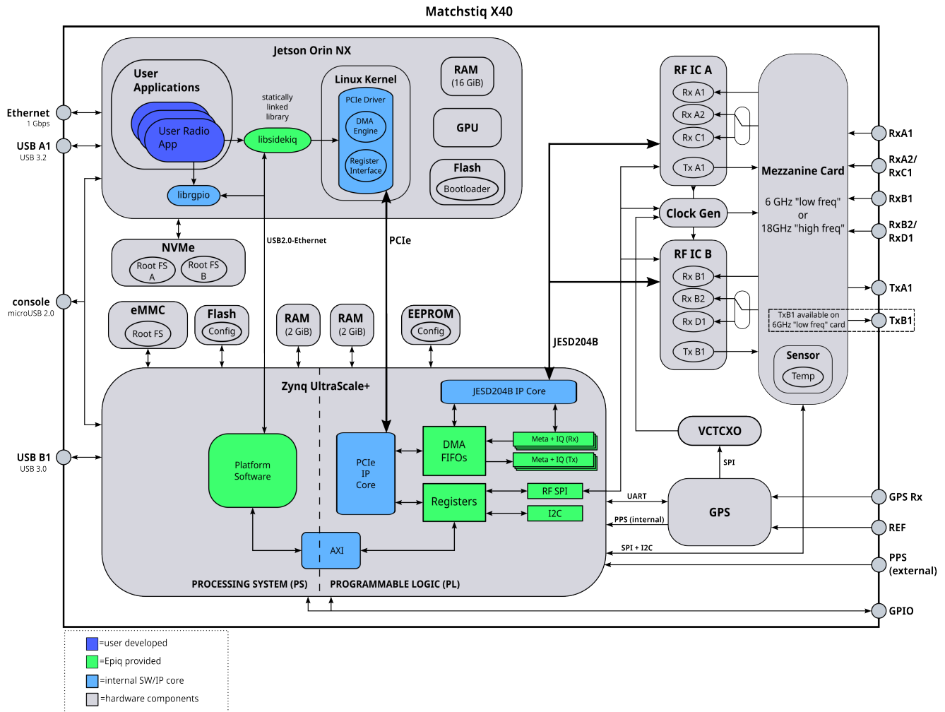
Fig. 4.11: Matchstiq X40 block diagram showing how libsideiq + user applications fit in the system
